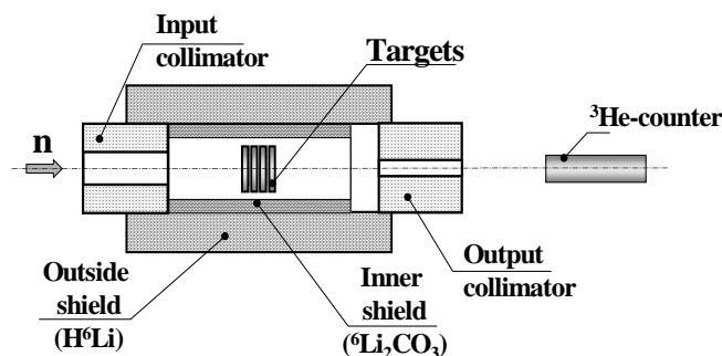
Fig. 4. Scheme of the radiation shielding system on the 2 nd HC and the target irradiation position.
