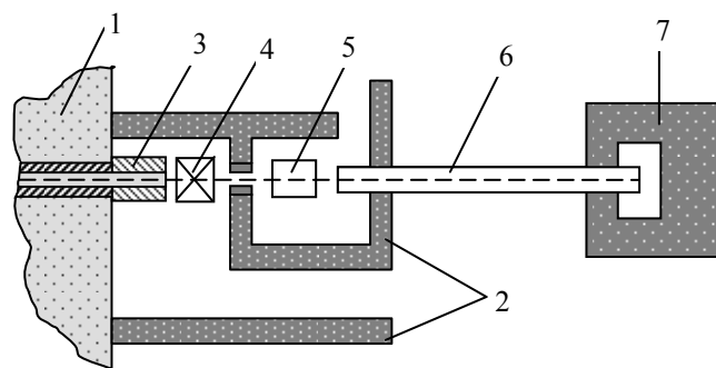
Fig. 3. Scheme of system of radiation shielding on the 8-th horizontal reactor channel. 1 – biological shielding; 2 – radiation shielding of installation; 3 – outside collimator; 4 – device for sample removing; 5 – neutron detector; 6 – tube for beam conducting up to neutron catching; 7 – neutron beam catching.
