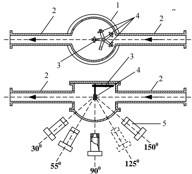
Fig. 6. Installation IASD-1: vacuum chamber scheme. 1 – chamber; 2 – neutron guide; 3 – sample changing gear ; 4 – sample-scatterer; 5 – neutron detector with preamplifier.
