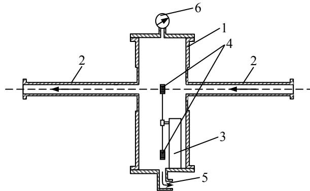
Fig. 7. Schematic view of vacuum chamber of IASD-2 installation: 1 – chamber; 2 – neutron guide; 3 – electromechanical device; 4 – sample-scatterers; 5 – vacuum socket; 6 – vacuum gage.
