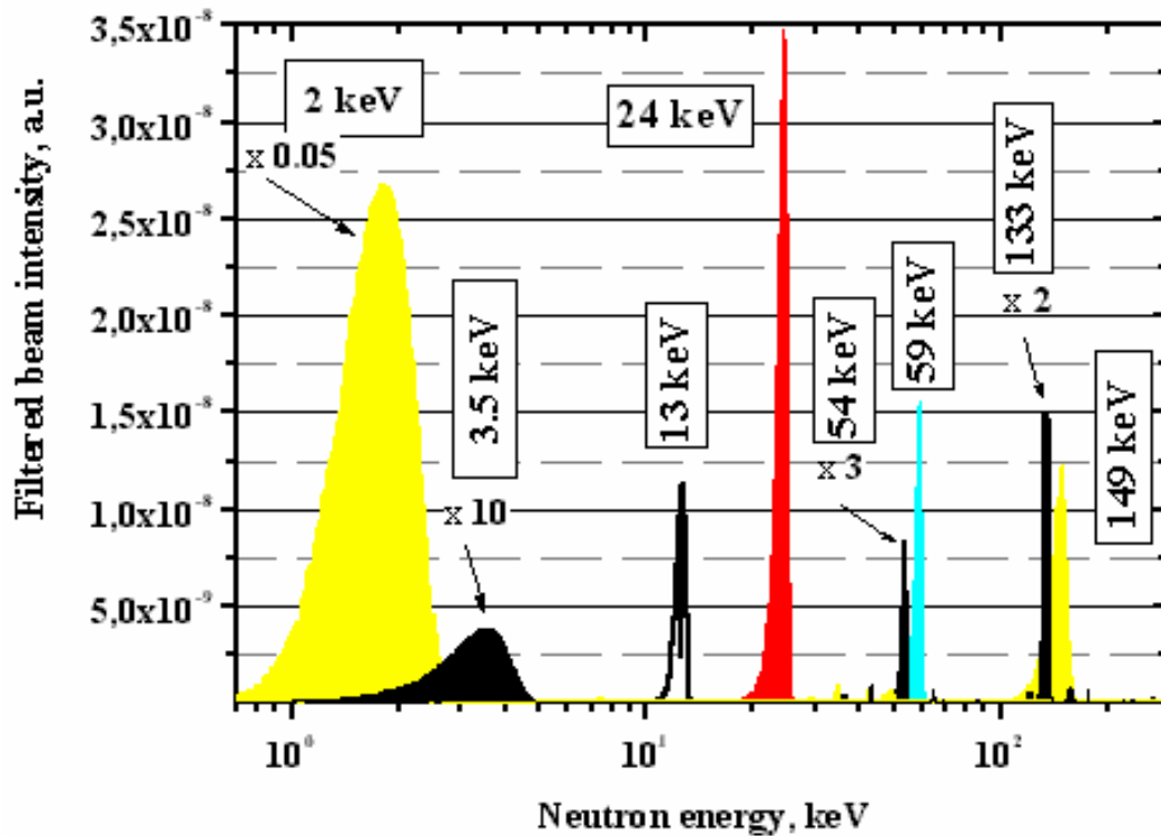
Fig. 1. Neutron filters used in the NPD for fundamental investigations.
