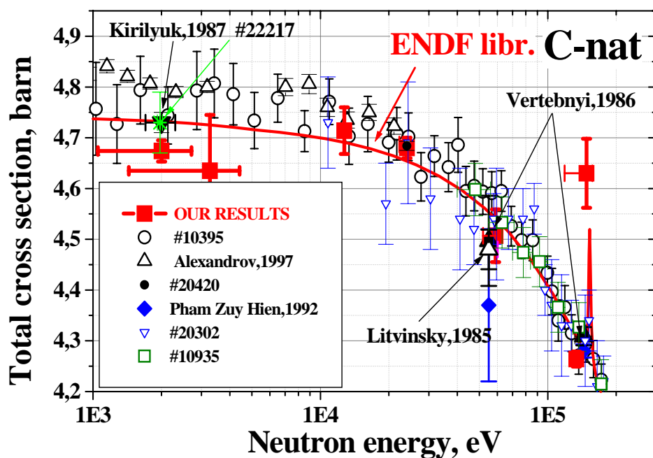
Fig. 9. Experimental results for the total neutron cross sections on carbon, obtained in NPD using transmission method [2, 3] and data from ENDFB/6 and EXFOR libraries.
