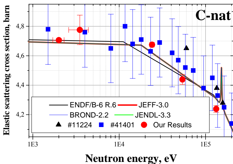
Fig. 10. Our results of the neutron scattering cross sections for natural carbon in the energy range 2 -133 keV [4, 5], the known experimental data from database EXFOR/CSISRS and ENDF libraries.
