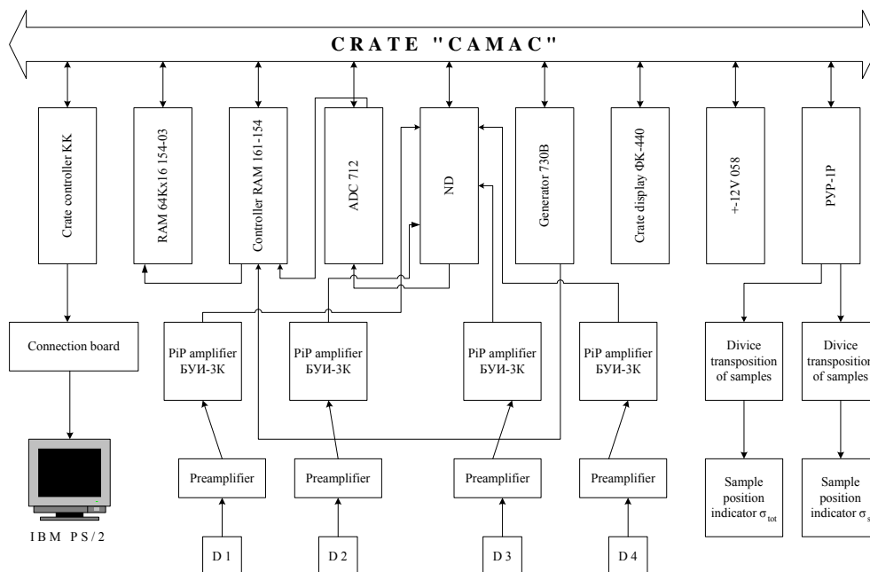
Fig 8. Flow block of spectrometry section in installation for differential cross section measurements.
