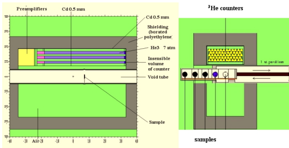
Fig. 5. Disposition of the He-3 counters and samples (vertical cross section). In the left - along neutron beam, in the right - perpendicular to beam.
