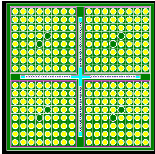
MCNP Computer Model of BWR Reactor Bundles
