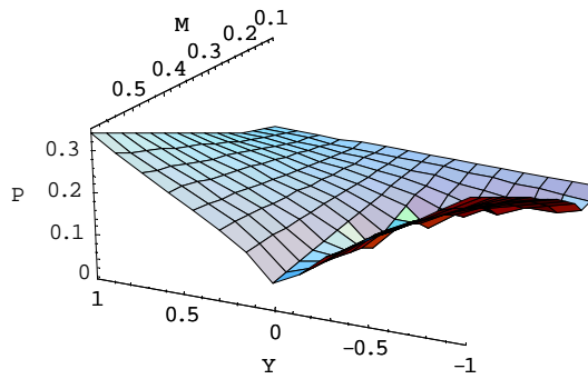
Figure 4. The shear stress P vs. M^* and Y at a=b=2.5
